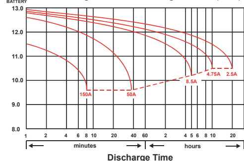
(N) FOR 12V BATTERY Discharge Time VS. Discharge Current (25°C)
